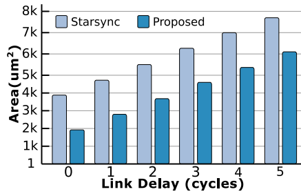
Fig. 6. Area occupied by the synchronizers as the delay of the link increases. In this comparison, the tightly coupled approach [9] is not included, because it does not support multicycle link delays.
